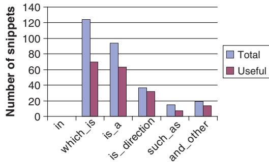
Fig. 8. Number of snippets and those containing at least one correct location (useful) by trigger phrase.
