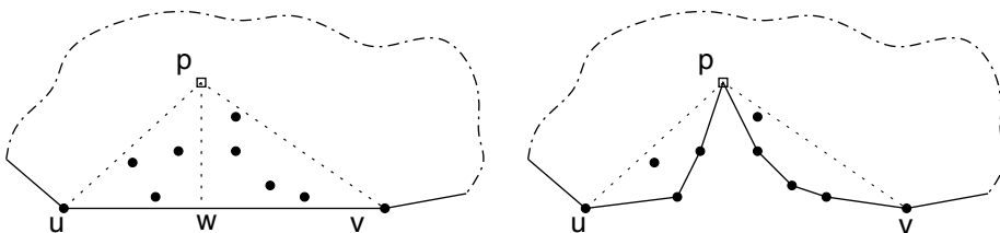
Fig. 3. Construction illustrating how a polygon is adapted so that the blue point p is no longer inside.
