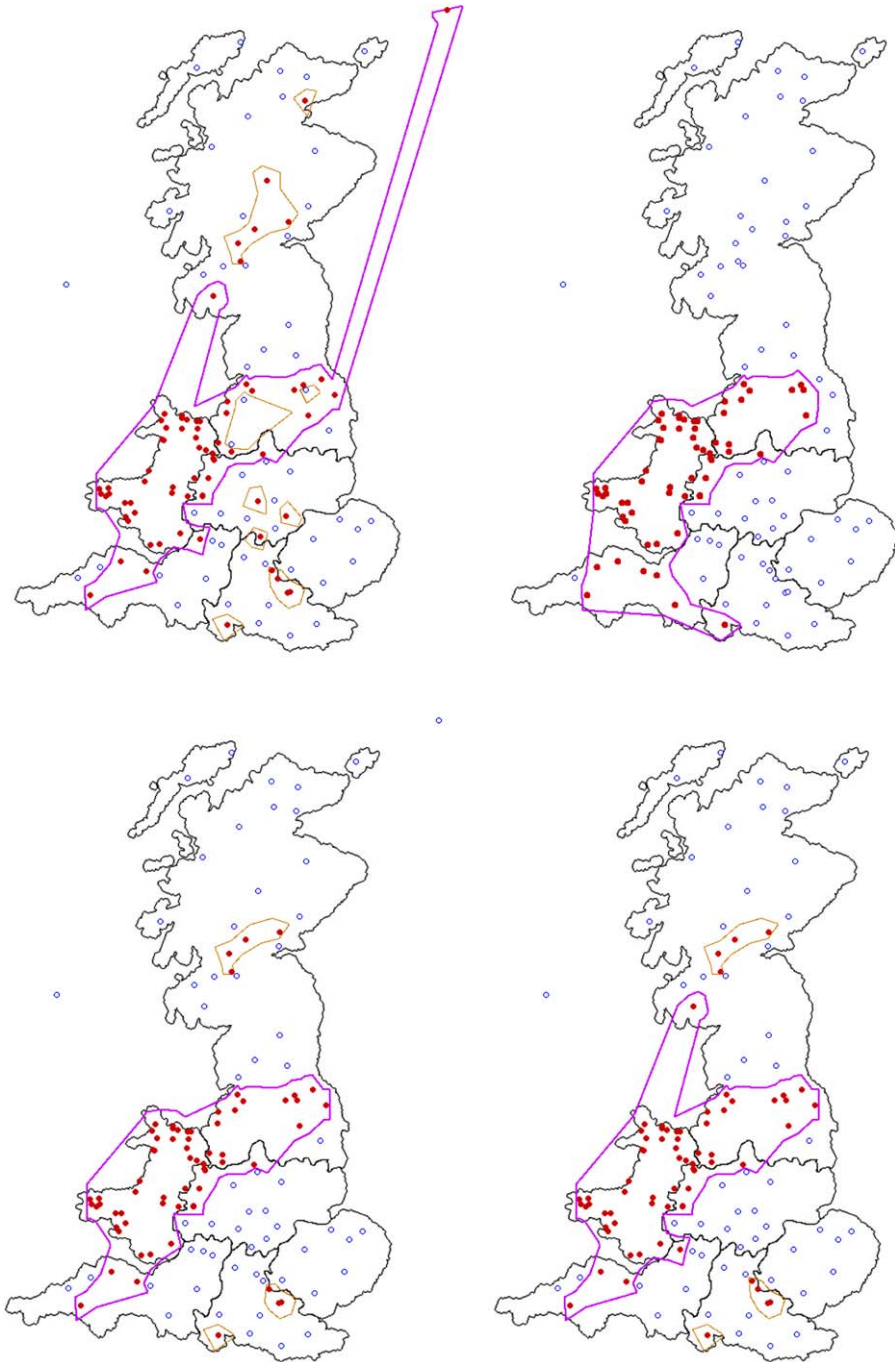
Fig. 11. Delineated polygon for Wales before recoloring, and the outcome of the recoloring algorithm with angles 185, 215, and 260.
