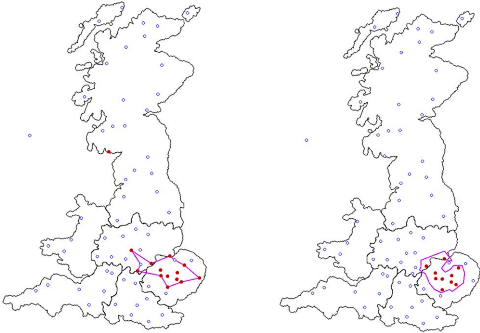
Fig. 13. Delineated polygon for East Anglia with the \alpha -shape algorithm ( \alpha = 600 ) and the recoloring method (angle 215).
