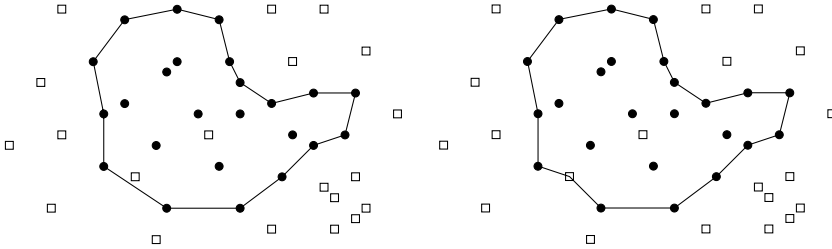
Fig. 2. \alpha -Shape of a set of red points (circles) and its adaptation so that a blue point (square) is no longer inside.
