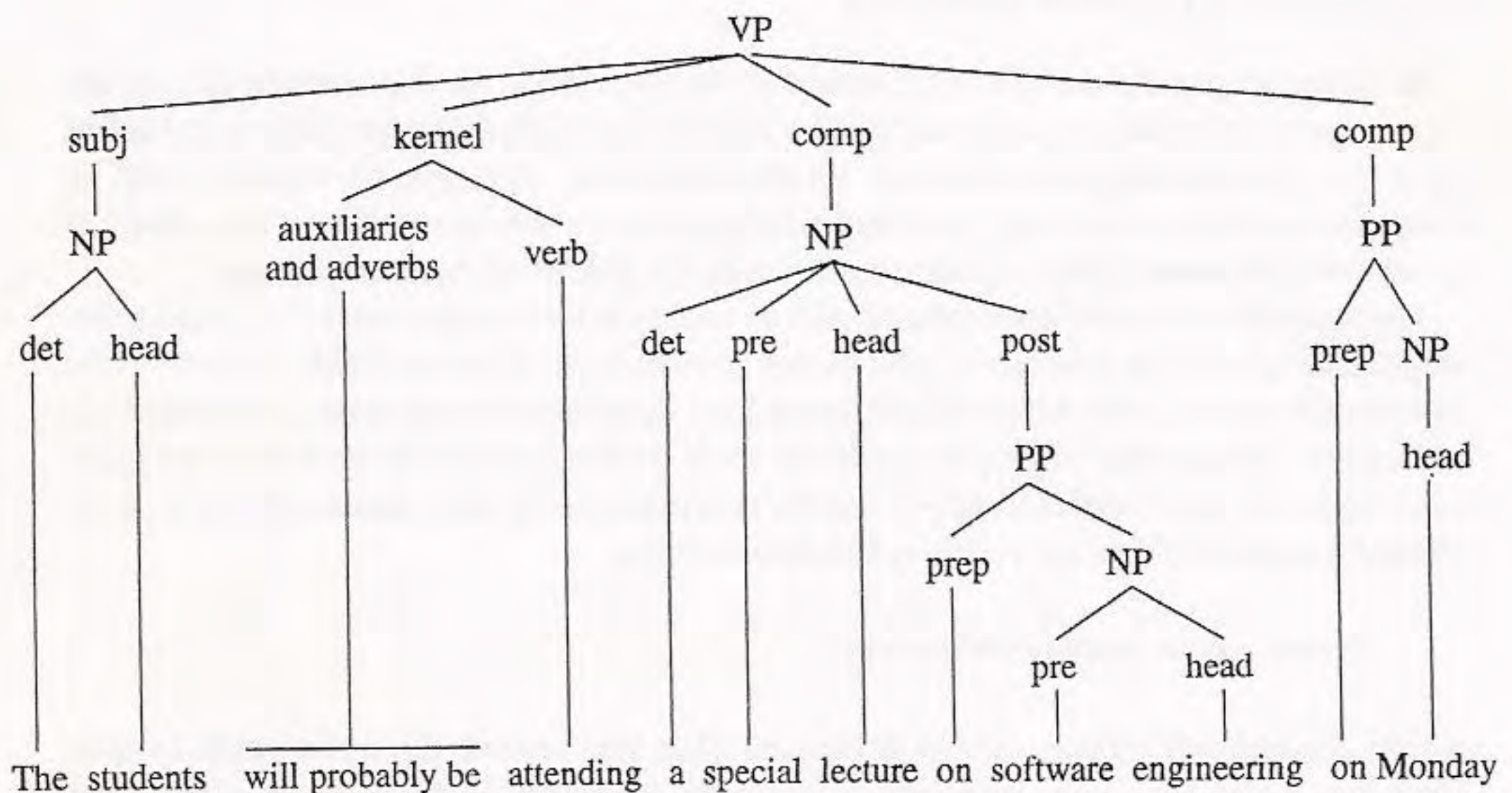
FIGURE 1. Light parsing for IR purposes.
